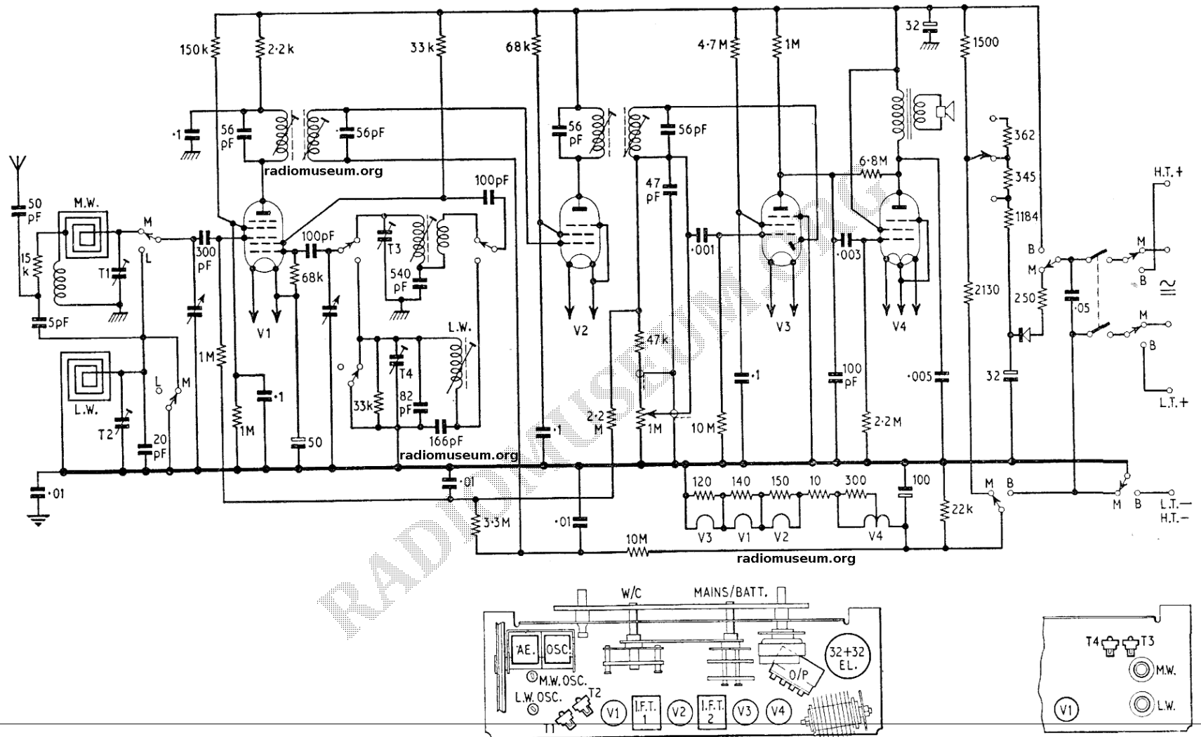
CIRCUIT DIAGRAM—EKCO "STROLLER III" MODEL MBP183
