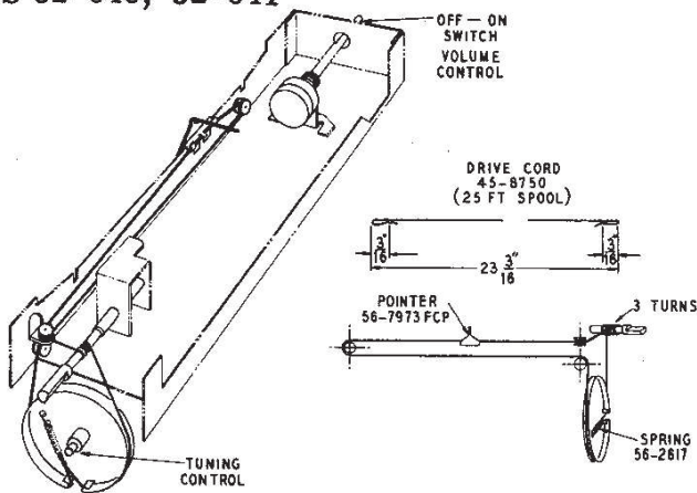
Figure 4. Drive-Cord-Installation Details
