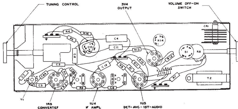
Figure 1. Bottom View, Showing Symbolized Chassis
