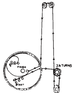
STRINGING DIAGRAM
